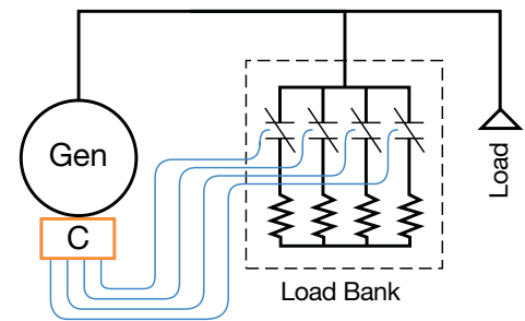
Single Generators with Special Emissions Requirements
