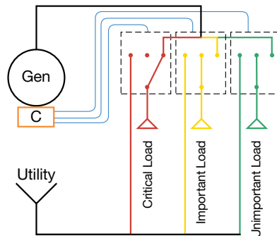
Single Generator Controlling ATS
