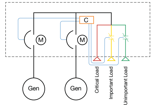
Parallel Generators with Load Management in Switchgear
