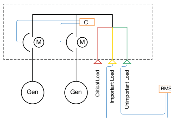
Parallel Generators with Building Management System (BMS)
