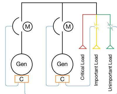
Parallel Generators with Load Management in Controller
