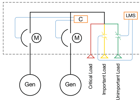
Parallel Generators with Load Management System (LMS)
